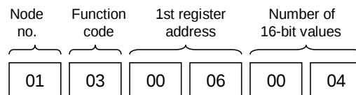
Figure 2 - ModBus Read Message Example
